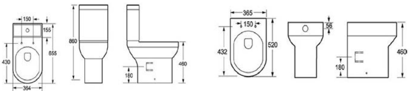
Comfort Height Open Back Pan
