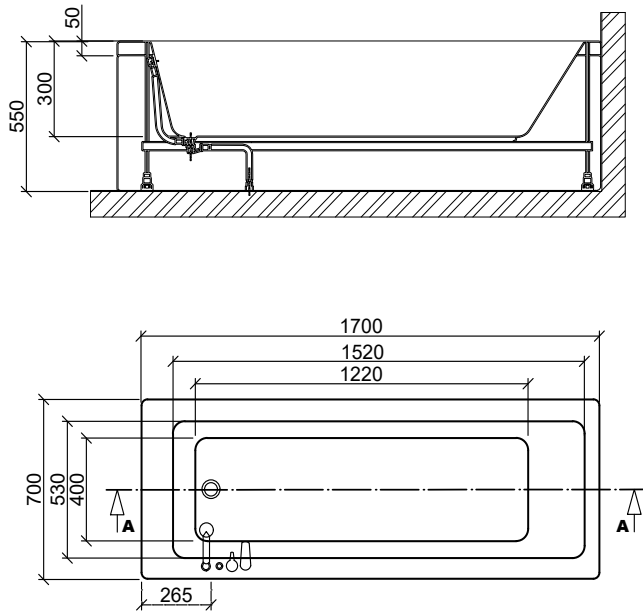
Single Ended Bath - 1700mm x 750mm
