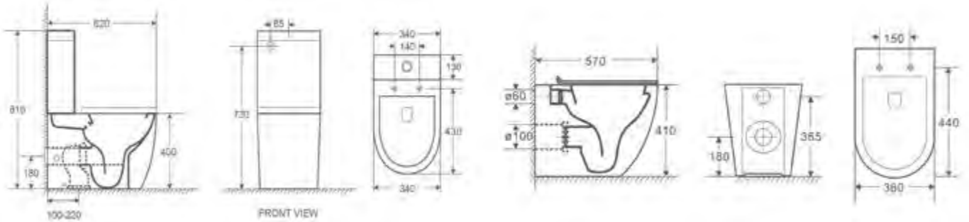
Rimless Fully Back To Wall Pan
